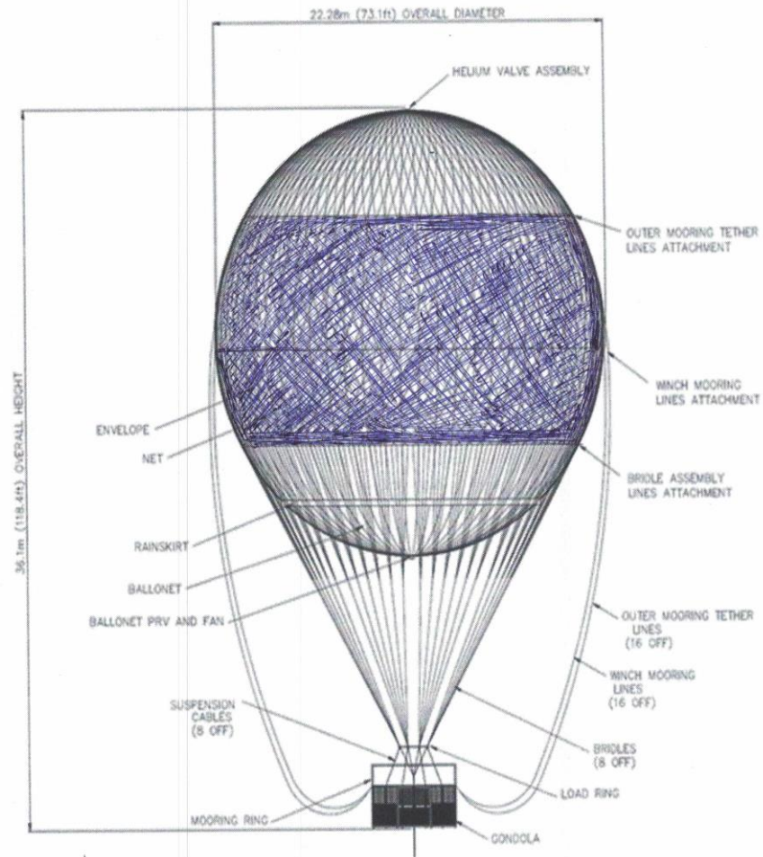
Figure 1: Balloon System
